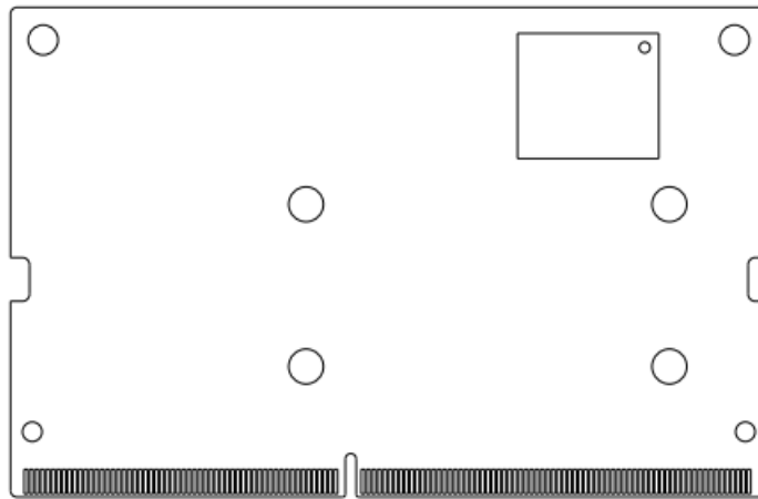
Figure 10 Module Bottom Showing EMMC Placement
