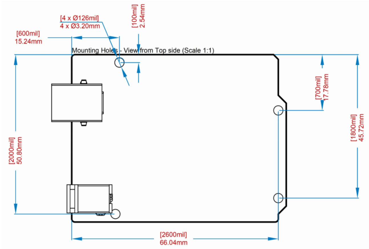
Board outline
